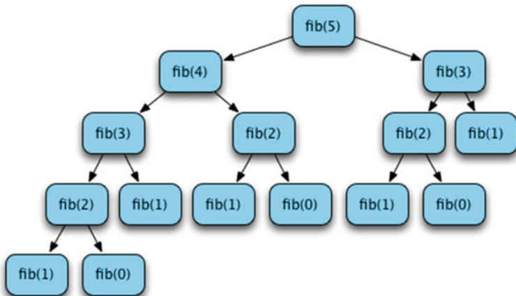
Fig. 5.7 Computing fib(5)
