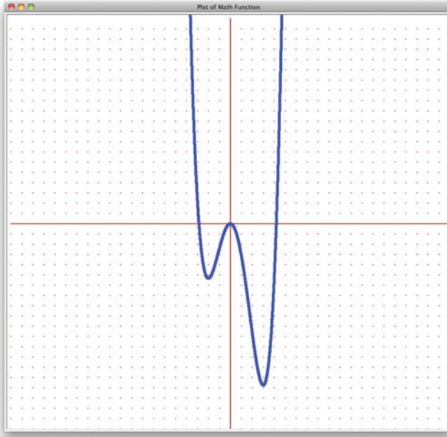
Fig. 4.5 The plot of g(x) = x^4/4 - x^3/3 - 3x^2
