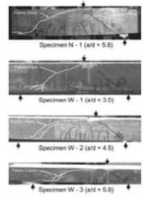
Fig. 13—Photographs of asymmetric tests after failure for all specimens a/d = 1.7 for right side; a/d ratios listed within figure refer to left side. ∞ failure occurred at the side with the large a/d, direct strut action for a/d = 1,7 but authors found this surprising Zsutty, T. (1971). "Shear Strength Prediction for Separate Categories of Simple Beam Tests." ACI Journal Proceedings , 68(2), 138-143. formula: v_u = 1670 (f'_c)^{0.26} p^{0.41} \left(\frac{d}{a}\right)^{1.50} as a/d decreases below 2.5, the short beam arch action of load and support blocks creates strengths greater than predicted with the equation for slender beams. The easiest way to take this into account would be through a linear arch action factor given by: limit of a/d for slender beam action/short beam a/d or arch description = 2.5/a/d \Rightarrow v_u = 150 (f'_c p)^{1/3} \left(\frac{d}{a}\right)^{1.3} Clark, A. P., 1951, "Diagonal Tension in Reinforced Concrete Beams." ACI Journal Proceedings , Vol. 48, No. 10, pp. 145-156. ∞ first to determine the position of the load as an important factor ∞ test data with small a/d < 2" the results of this study with tests under five different loading conditions show definitely that the loading condition is an important factor
