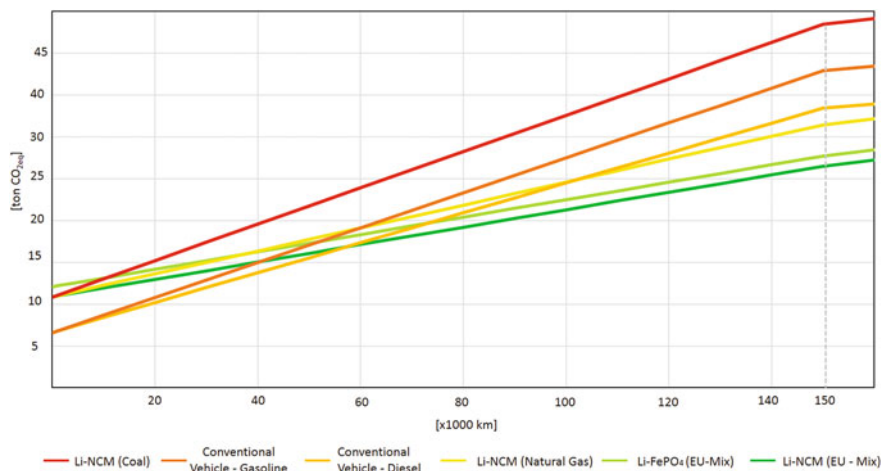
Fig. 27.8 Comparison of the life cycle GWP of a CV and an EV as function of the distance driven
