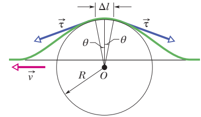
Figure 16-9 A symmetrical pulse, viewed from a reference frame in which the pulse is stationary and the string appears to move right to left with speed v . We find speed v by applying Newton's second law to a string element of length \Delta l , located at the top of the pulse.
