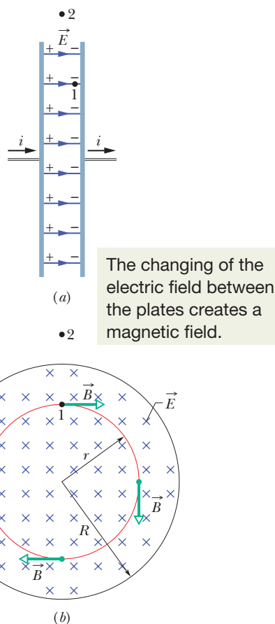
Figure 32-5 (a) A circular parallel-plate capacitor, shown in side view, is being charged by a constant current i . (b) A view from within the capacitor, looking toward the plate at the right in (a). The electric field \vec{E} is uniform, is directed into the page (toward the plate), and grows in magnitude as the charge on the capacitor increases. The magnetic field \vec{B} induced by this changing electric field is shown at four points on a circle with a radius r less than the plate radius R .
