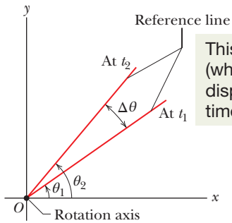
Figure 10-4 The reference line of the rigid body of Figs. 10-2 and 10-3 is at angular position \theta_1 at time t_1 and at angular position \theta_2 at a later time t_2 . The quantity \Delta\theta (= \theta_2 - \theta_1) is the angular displacement that occurs during the interval \Delta t (= t_2 - t_1) . The body itself is not shown.
