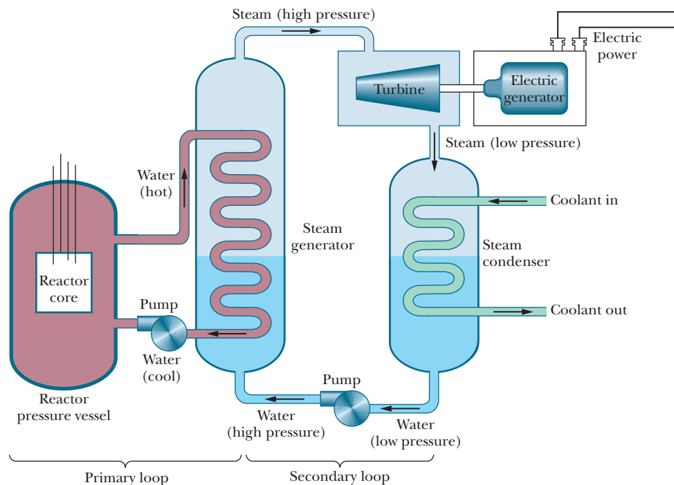
Figure 43-6 A simplified layout of a nuclear power plant, based on a pressurized-water reactor. Many features are omitted — among them the arrangement for cooling the reactor core in case of an emergency.
