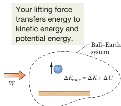
Figure 8-12 Positive work W is done on a system of a bowling ball and Earth, causing a change \Delta E_{\text{mec}} in the mechanical energy of the system, a change \Delta K in the ball's kinetic energy, and a change \Delta U in the system's gravitational potential energy.
