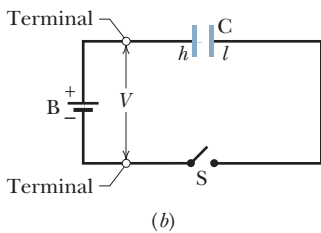
Figure 25-4 (a) Battery B, switch S, and plates h and l of capacitor C, connected in a circuit. (b) A schematic diagram with the circuit elements represented by their symbols.
