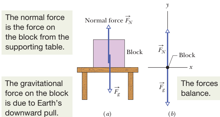
Figure 5-7 (a) A block resting on a table experiences a normal force \vec{F}_N perpendicular to the tabletop. (b) The free-body diagram for the block.
