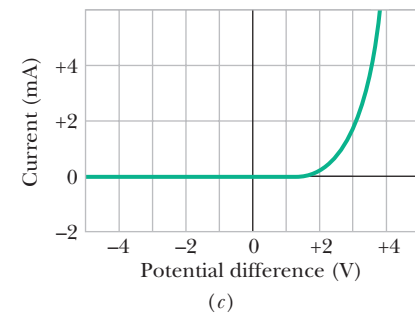
Figure 26-11 (a) A potential difference V is applied to the terminals of a device, establishing a current i . (b) A plot of current i versus applied potential difference V when the device is a 1000\ \Omega resistor. (c) A plot when the device is a semiconducting pn junction diode.
