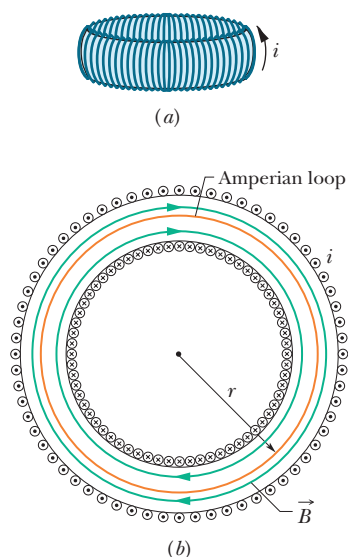
Figure 29-21 (a) A toroid carrying a current i . (b) A horizontal cross section of the toroid. The interior magnetic field (inside the bracelet-shaped tube) can be found by applying Ampere's law with the Amperian loop shown.
