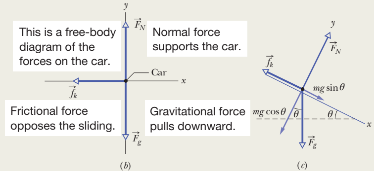
Figure 6-4 (a) A car sliding to the right and finally stopping. A free-body diagram for the car on (b) the same horizontal road and (c) a hill.
