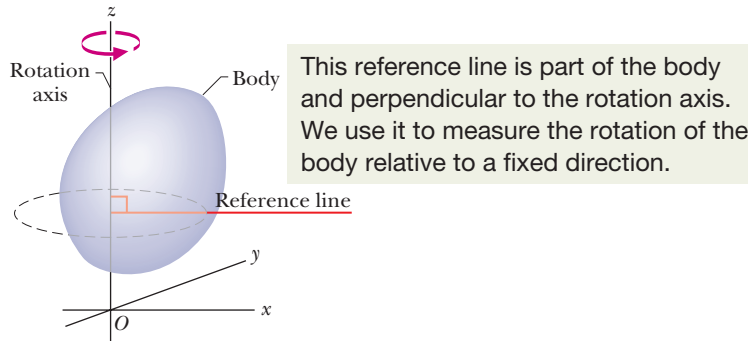
Figure 10-2 A rigid body of arbitrary shape in pure rotation about the z axis of a coordinate system. The position of the reference line with respect to the rigid body is arbitrary, but it is perpendicular to the rotation axis. It is fixed in the body and rotates with the body.
