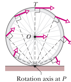
Figure 11-6 Rolling can be viewed as pure rotation, with angular speed \omega , about an axis that always extends through P . The vectors show the instantaneous linear velocities of selected points on the rolling wheel. You can obtain the vectors by combining the translational and rotational motions as in Fig. 11-4.
