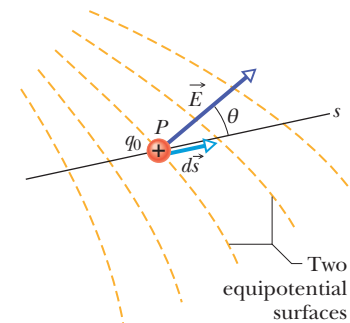
Figure 24-17 A test charge q_0 moves a distance d\vec{s} from one equipotential surface to another. (The separation between the surfaces has been exaggerated for clarity.) The displacement d\vec{s} makes an angle \theta with the direction of the electric field \vec{E} .
