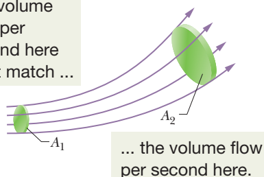
Figure 14-17 A tube of flow is defined by the streamlines that form the boundary of the tube. The volume flow rate must be the same for all cross sections of the tube of flow.
