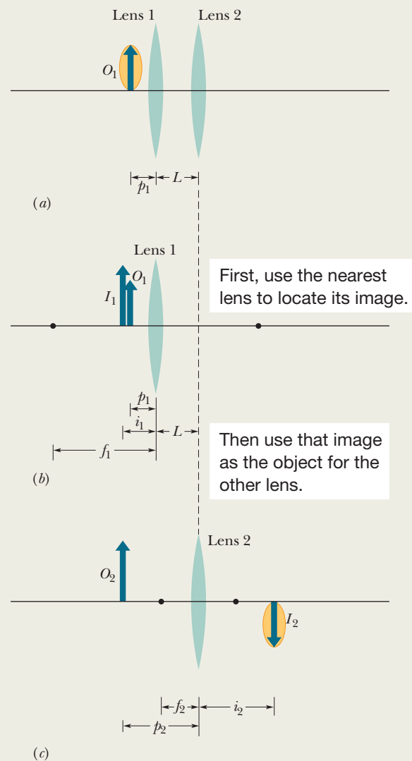
Figure 34-18 (a) Seed O_1 is distance p_1 from a two-lens system with lens separation L . We use the arrow to orient the seed. (b) The image I_1 produced by lens 1 alone. (c) Image I_1 acts as object O_2 for lens 2 alone, which produces the final image I_2 .
