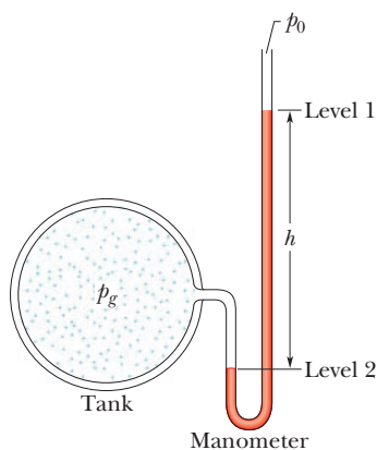
Figure 14-6 An open-tube manometer, connected to measure the gauge pressure of the gas in the tank on the left. The right arm of the U-tube is open to the atmosphere.
