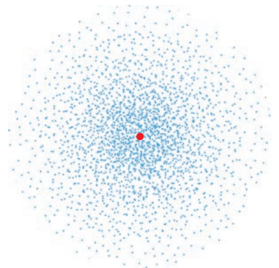
Figure 39-20 A “dot plot” showing the volume probability density \psi^2(r) — not the radial probability density P(r) — for the ground state of the hydrogen atom. The density of dots drops exponentially with increasing distance from the nucleus, which is represented here by a red spot.
