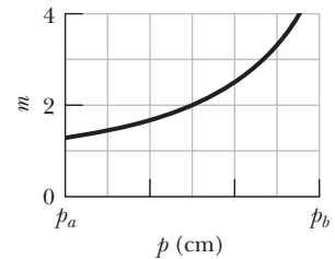
Figure 34-35 Problem 6.
