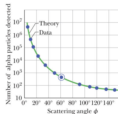
Figure 42-2 The dots are alpha-particle scattering data for a gold foil, obtained by Geiger and Marsden using the apparatus of Fig. 42-1. The solid curve is the theoretical prediction, based on the assumption that the atom has a small, massive, positively charged nucleus. The data have been adjusted to fit the theoretical curve at the experimental point that is enclosed in a circle.
