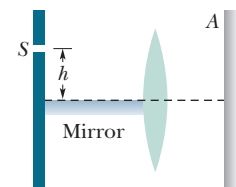
Figure 35-60 Problem 104.
