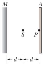
Figure 34-32 Problem 3.
