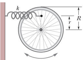
Figure 15-52 Problem 70.
