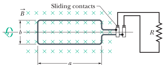
Figure 30-40 Problem 11.
