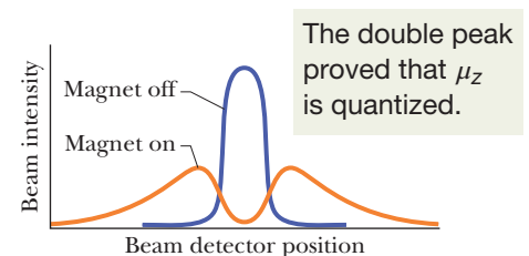
Figure 40-9 Results of a modern repetition of the Stern–Gerlach experiment. With the electromagnet turned off, there is only a single beam; with the electromagnet turned on, the original beam splits into two subbeams. The two subbeams correspond to parallel and antiparallel alignment of the magnetic moments of cesium atoms with the external magnetic field.
