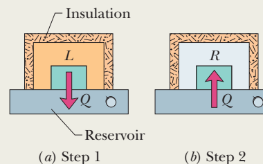
Figure 20-6 The blocks of Fig. 20-5 can proceed from their initial state to their final state in a reversible way if we use a reservoir with a controllable temperature (a) to extract heat reversibly from block L and (b) to add heat reversibly to block R .
