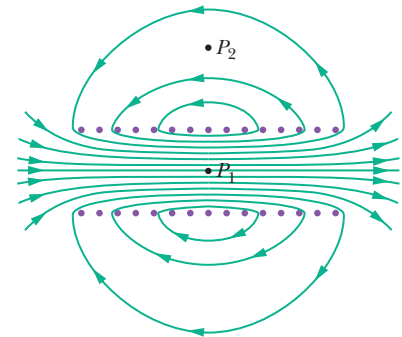
Figure 29-19 Magnetic field lines for a real solenoid of finite length. The field is strong and uniform at interior points such as P_1 but relatively weak at external points such as P_2 .
