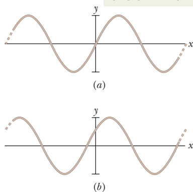
Figure 16-6 A sinusoidal traveling wave at t = 0 with a phase constant \phi of (a) 0 and (b) \pi/5 rad.
