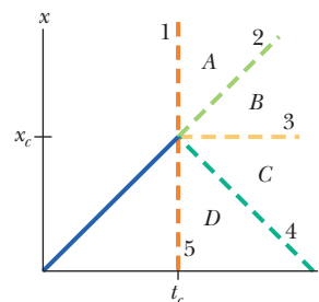
Figure 9-33 Question 11.
