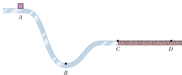
Figure 8-22 Question 5.
