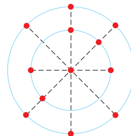
Figure 13-23 Question 3.
