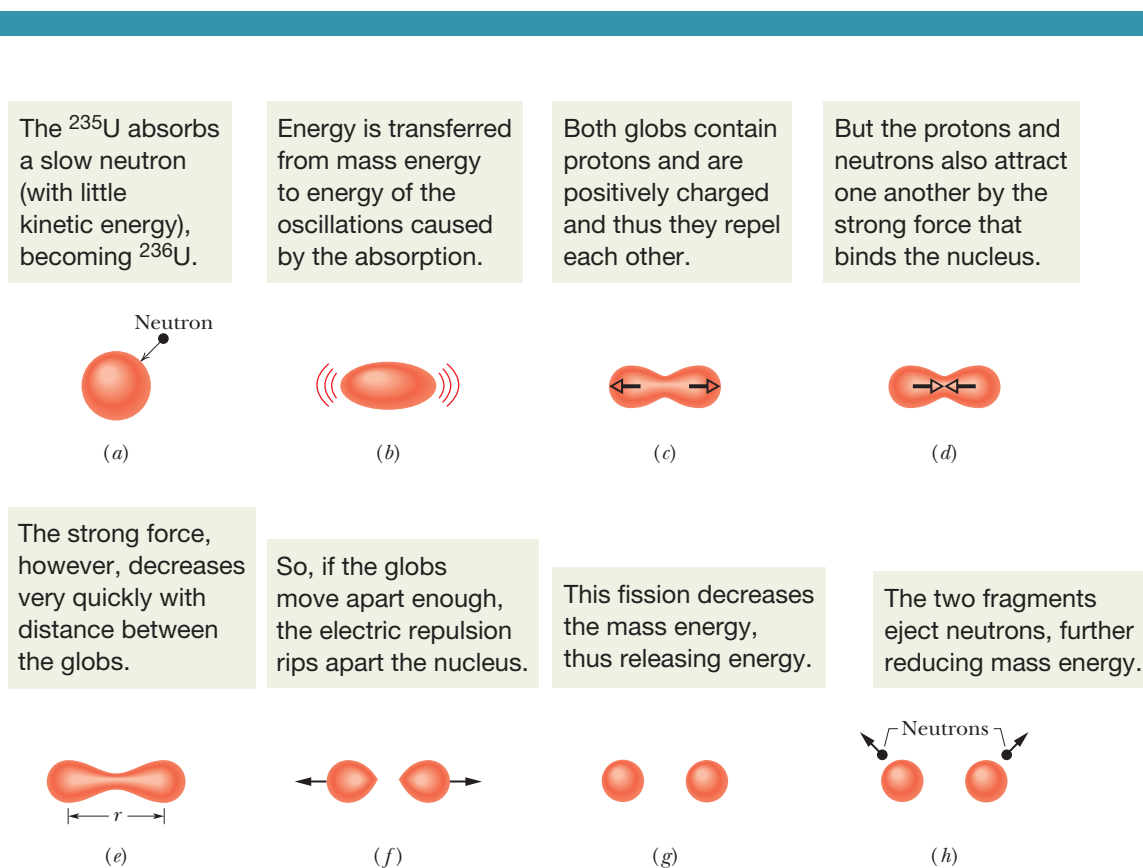
Figure 43-2 The stages of a typical fission process, according to the collective model of Bohr and Wheeler.
