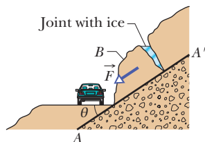
Figure 6-22 Problem 14.
