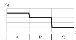
Figure 26-22 Question 9.
