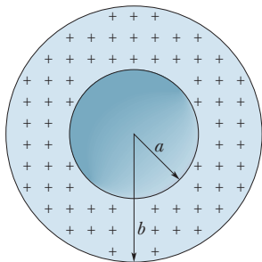
Figure 23-57 Problem 52.
