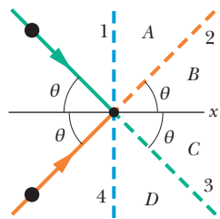
Figure 9-73 Problem 84.
