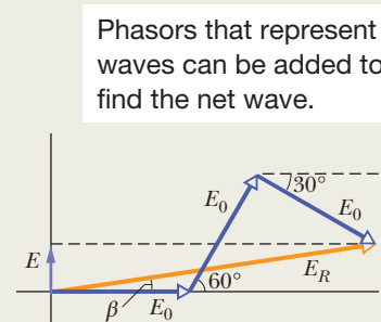
Figure 35-14 Three phasors, representing waves with equal amplitudes E_0 and with phase constants 0^\circ , 60^\circ , and -30^\circ , shown at time t = 0 . The phasors combine to give a resultant phasor with magnitude E_R , at angle \beta .
