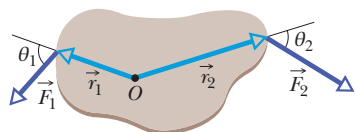
Figure 10-39 Problem 45.
