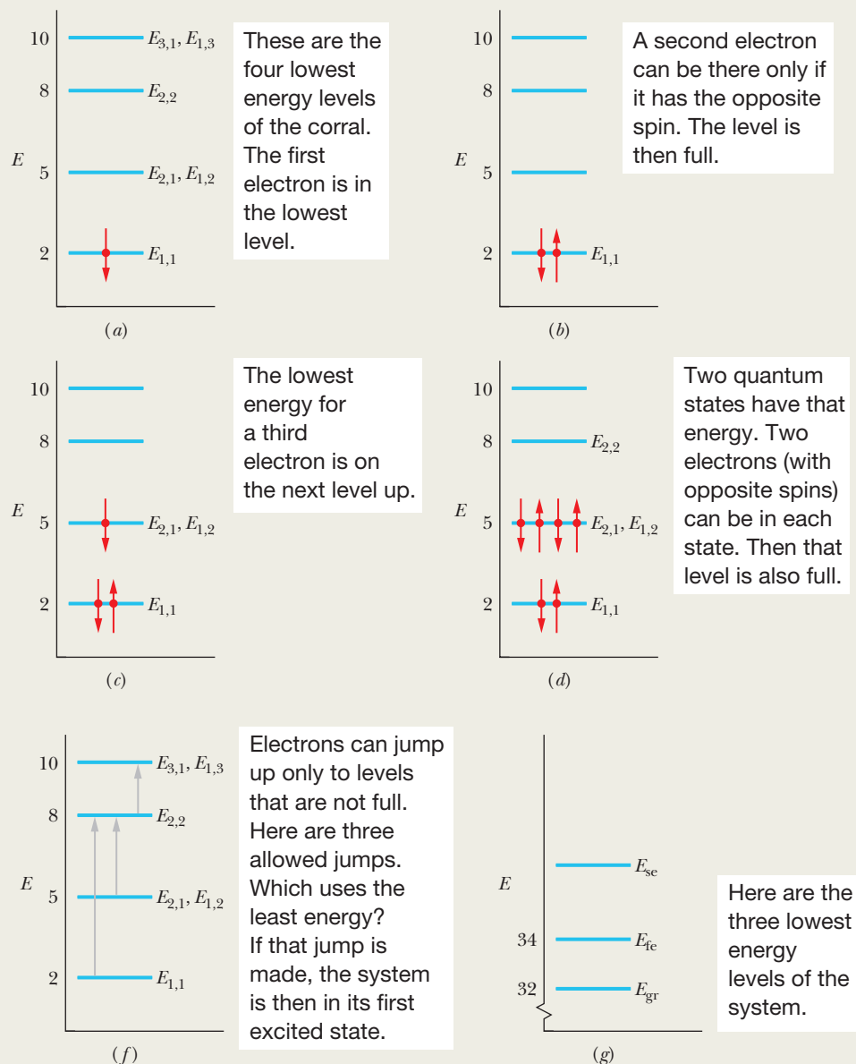
Figure 40-12 (a) Energy-level diagram for one electron in a square corral. (Energy E is in multiples of h^2/8mL^2 .) A spin-down electron occupies the lowest level. (b) Two electrons (one spin down, the other spin up) occupy the lowest level of the one-electron energy-level diagram. (c) A third electron occupies the next energy level. (d) Four electrons can be put into the second level. (e) The system's ground-state configuration. (f) Three transitions to consider for the first excited state. (g) The system's lowest three total energies.
