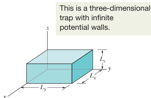
Figure 39-14 A rectangular box — a three-dimensional version of the infinite potential well of Fig. 39-2 — with widths L_x , L_y , and L_z .
