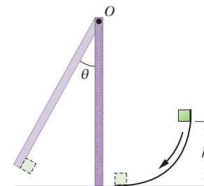
Figure 11-58 Problem 66.
