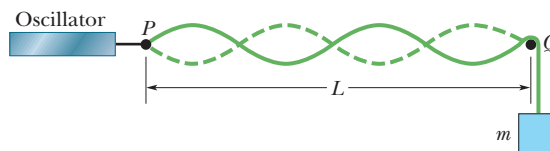
Figure 16-42 Problems 58 and 60.
