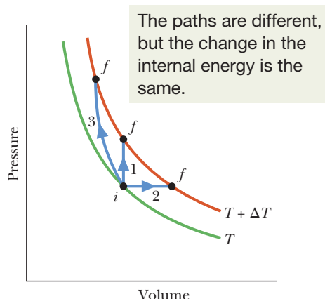
Figure 19-10 Three paths representing three different processes that take an ideal gas from an initial state i at temperature T to some final state f at temperature T + \Delta T . The change \Delta E_{\text{int}} in the internal energy of the gas is the same for these three processes and for any others that result in the same change of temperature.
