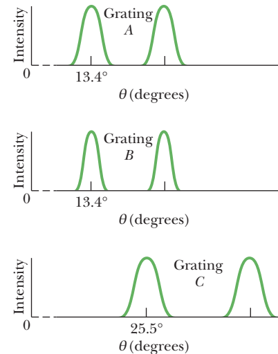
Figure 36-26 The intensity patterns for light of two wavelengths sent through the gratings of Table 36-1. Grating B has the highest resolving power, and grating C has the highest dispersion.
