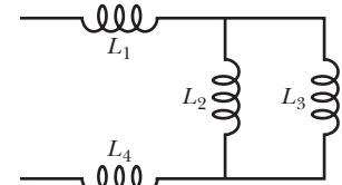
Figure 30-61 Problem 49.
