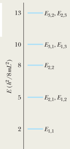
Figure 39-15 Energy-level diagram for an electron trapped in a square corral.
