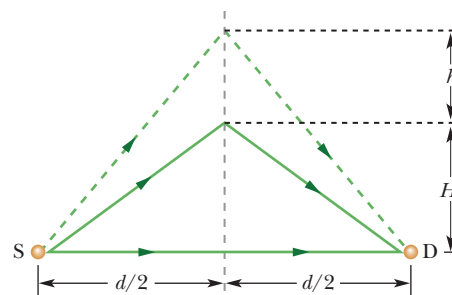
Figure 17-52 Problem 108.
