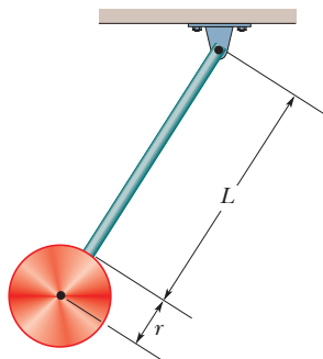
Figure 15-42 Problem 41.
