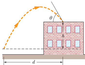
Figure 4-41 Problem 48.
