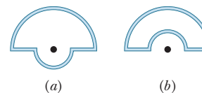
Figure 29-47 Problem 18.
