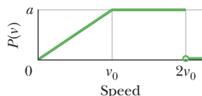
Figure 19-23 Problem 37.
