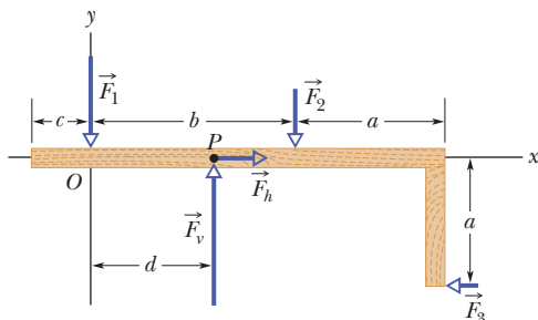
Figure 12-33 Problem 15.
