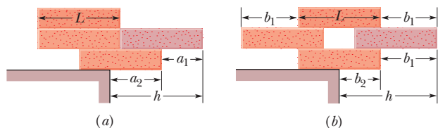
Figure 12-83 Problem 79.
