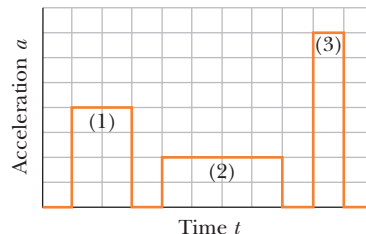
Figure 2-23 Question 11.
