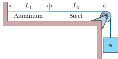
Figure 16-43 Problem 59.
