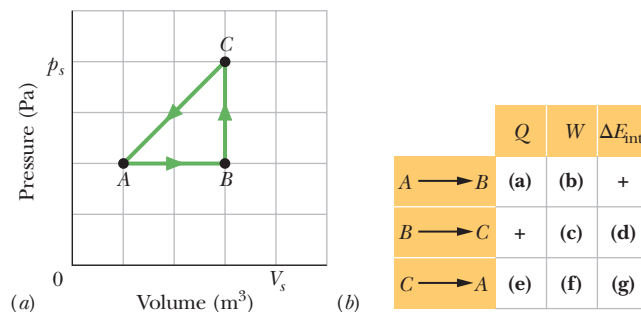
Figure 18-38 Problem 44.
