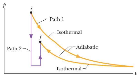
Figure 19-26 Problem 59.
