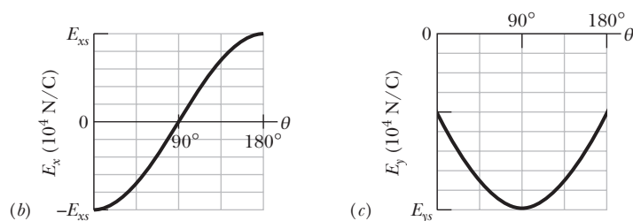
Figure 22-44 Problem 17.
