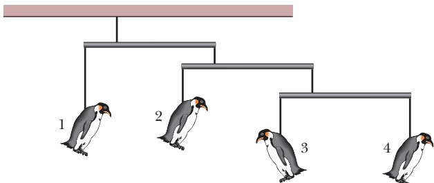
Figure 12-18 Question 5.
