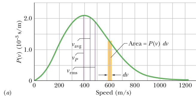
Figure 19-8 (a) The Maxwell speed distribution for oxygen molecules at T = 300 \text{ K} . The three characteristic speeds are marked. (b) The curves for 300 \text{ K} and 80 \text{ K} . Note that the molecules move more slowly at the lower temperature. Because these are probability distributions, the area under each curve has a numerical value of unity.
