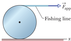
Figure 11-60 Problem 71.
