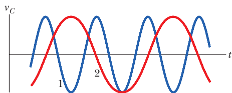
Figure 31-20 Question 2.
