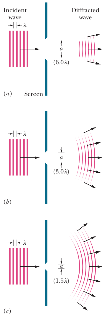
Figure 35-7 Diffraction represented schematically. For a given wavelength \lambda , the diffraction is more pronounced the smaller the slit width a . The figures show the cases for (a) slit width a = 6.0\lambda , (b) slit width a = 3.0\lambda , and (c) slit width a = 1.5\lambda . In all three cases, the screen and the length of the slit extend well into and out of the page, perpendicular to it.
