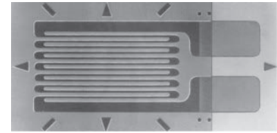
Figure 12-14 A strain gage of overall dimensions 9.8 mm by 4.6 mm. The gage is fastened with adhesive to the object whose strain is to be measured; it experiences the same strain as the object. The electrical resistance of the gage varies with the strain, permitting strains up to 3% to be measured.
