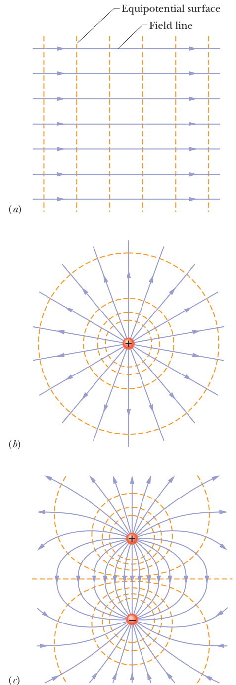
Figure 24-5 Electric field lines (purple) and cross sections of equipotential surfaces (gold) for (a) a uniform electric field, (b) the field due to a charged particle, and (c) the field due to an electric dipole.
