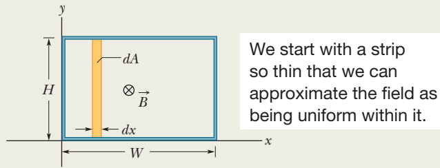
Figure 30-7 A closed conducting loop, of width W and height H , lies in a nonuniform, varying magnetic field that points directly into the page. To apply Faraday's law, we use the vertical strip of height H , width dx , and area dA .
