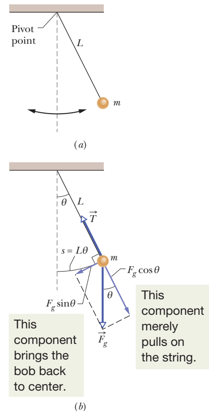
Figure 15-11 (a) A simple pendulum. (b) The forces acting on the bob are the gravitational force \vec{F}_g and the force \vec{T} from the string. The tangential component F_g \sin \theta of the gravitational force is a restoring force that tends to bring the pendulum back to its central position.
