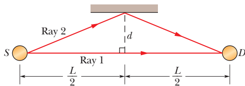
Figure 17-46 Problem 79.
