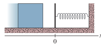
Figure 8-53 Problem 55.
