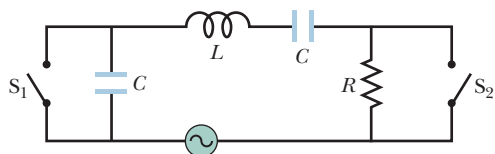
Figure 31-32 Problem 48.
