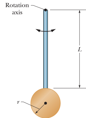
Figure 15-56 Problem 92.
