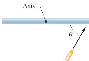
Figure 11-50 Problem 53.
