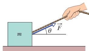
Figure 5-45 Problems 49 and 60.
