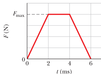
Figure 9-53 Problem 35.
