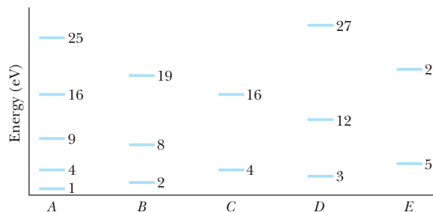
Figure 39-26 Question 14.
