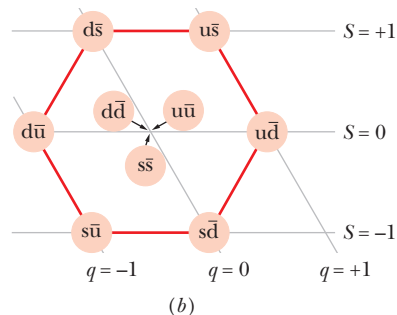
Figure 44-4 (a) The quark compositions of the eight spin- \frac{1}{2} baryons plotted in Fig. 44-3a. (Although the two central baryons share the same quark structure, they are different particles. The sigma is an excited state of the lambda, decaying into the lambda by emission of a gamma-ray photon.) (b) The quark compositions of the nine spin-zero mesons plotted in Fig. 44-3b.
