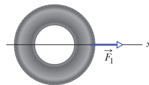
Figure 5-62 Problem 75.
