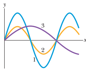
Figure 16-26 Question 4.
