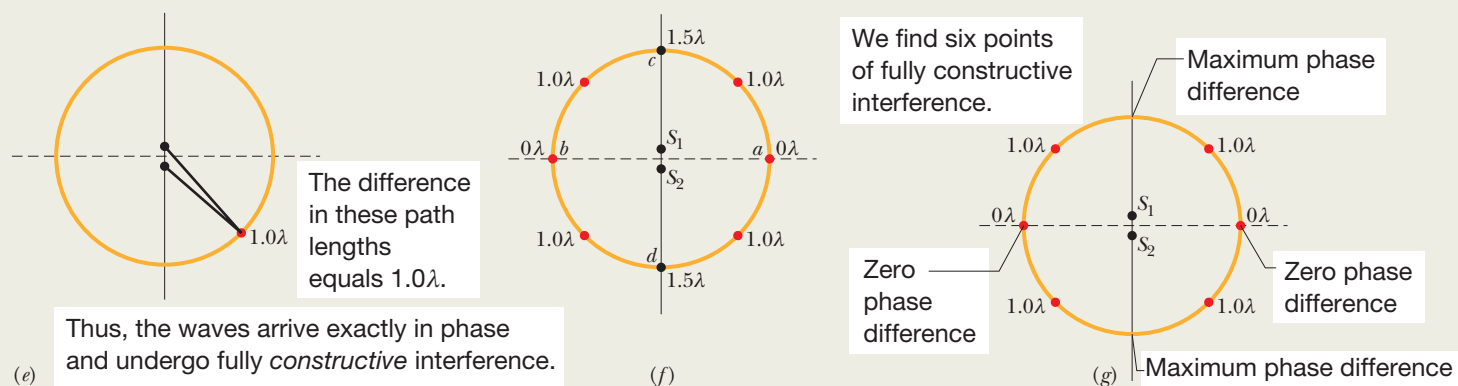
Figure 17-8 (continued) (e) Another point of fully constructive interference. (f) Using symmetry to determine other points. (g) The six points of fully constructive interference.
