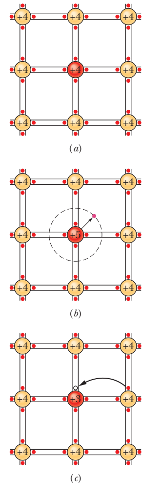
Figure 41-10 (a) A flattened-out representation of the lattice structure of pure silicon. Each silicon ion is coupled to its four nearest neighbors by a two-electron covalent bond (represented by a pair of red dots between two parallel black lines). The electrons belong to the bond — not to the individual atoms — and form the valence band of the sample. (b) One silicon atom is replaced by a phosphorus atom (valence = 5). The “extra” electron is only loosely bound to its ion core and may easily be elevated to the conduction band, where it is free to wander through the volume of the lattice. (c) One silicon atom is replaced by an aluminum atom (valence = 3). There is now a hole in one of the covalent bonds and thus in the valence band of the sample. The hole can easily migrate through the lattice as electrons from neighboring bonds move in to fill it. Here the hole migrates rightward.
