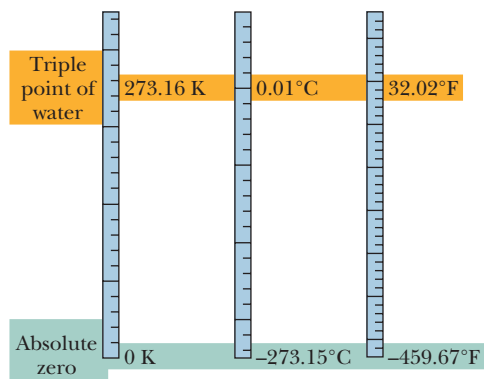
Figure 18-7 The Kelvin, Celsius, and Fahrenheit temperature scales compared.
