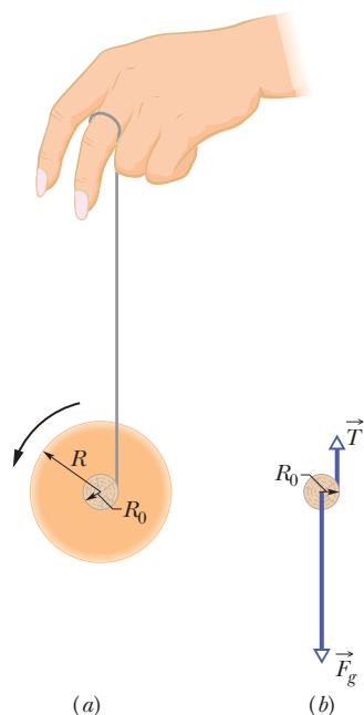
Figure 11-9 (a) A yo-yo, shown in cross section. The string, of assumed negligible thickness, is wound around an axle of radius R_0 . (b) A free-body diagram for the falling yo-yo. Only the axle is shown.
